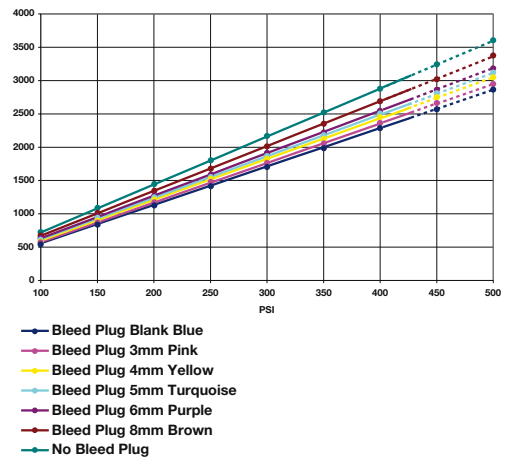
Dominator 1000 Air Consumption
